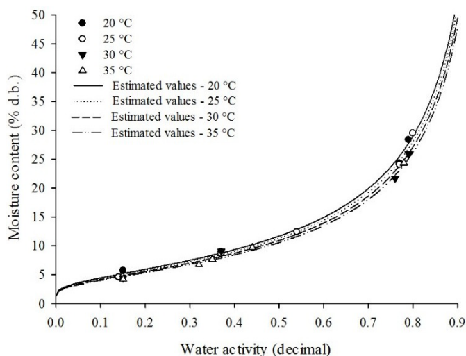
Figure 1. Experimental values of equilibrium moisture content and desorption isotherms estimated by the Modified Halsey model for baru fruits ( Dipteryx alata Vogel), under different conditions of temperature and water activity
