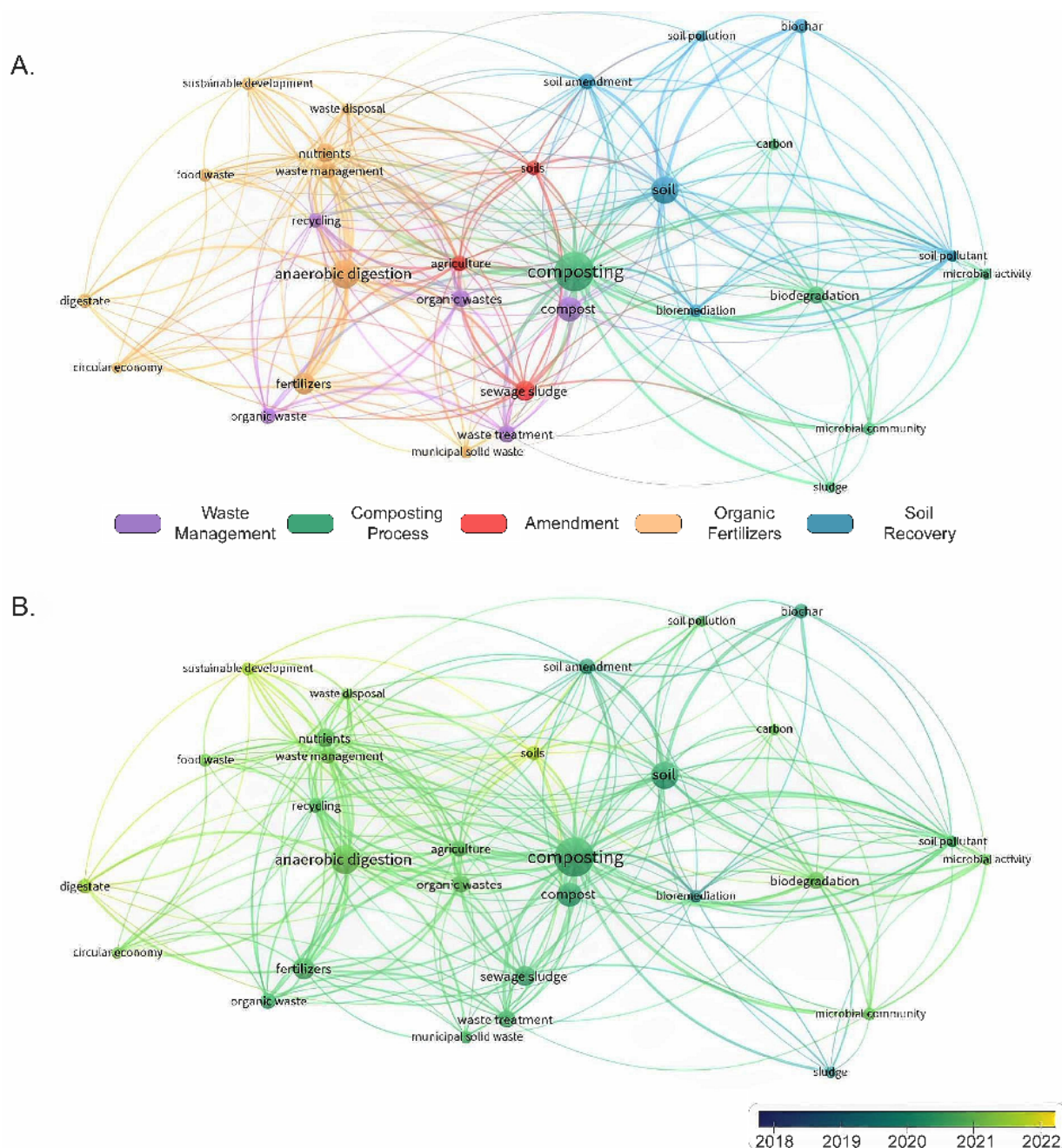
Figure 1. Maps of keywords co-occurrence in the selected articles (A) and chronological map with the most popular topics published between 2018 and 2022 (B)
